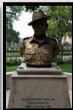
1962
